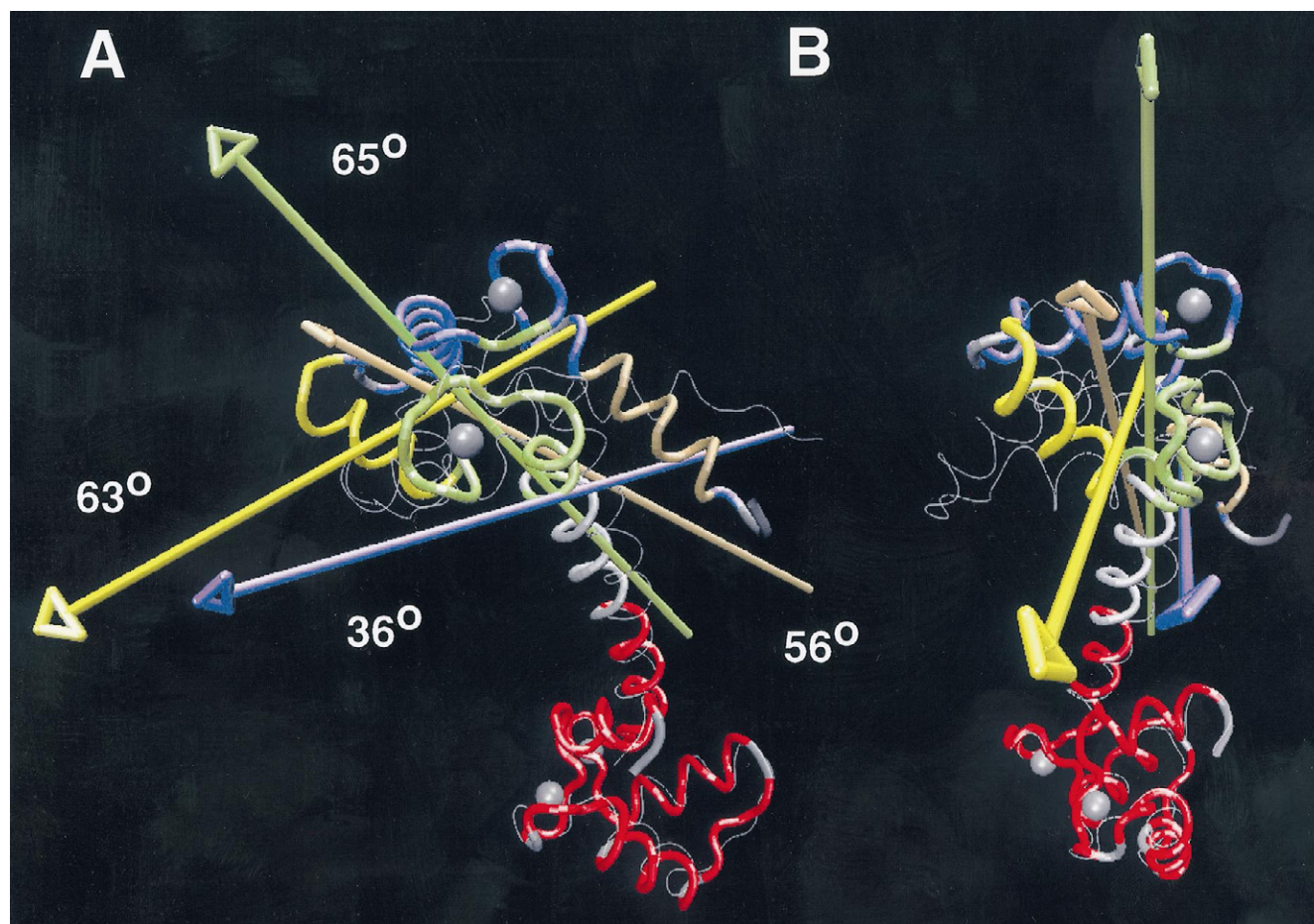
FIGURE 6 Domain movements of simulated structure ( A , side view; B , front view). The colored tube represents the structure after 3 ns (averaged over the last 20 ps) compared to the initial crystal structure (white line). Five rigid domains of more than 10 residues were extracted by Hingefind (Wriggers and Schulten, 1997) partitioning at 2.0 Å resolution. Domain 1 (red), the reference domain, comprises 63 residues located in the C-terminal domain. The movements of the four subdomains in the N-terminal lobe were visualized by the effective rotation axes relative to the C-terminal lobe. The arrows indicate a left-handed rotation from the initial to the final structure. Domain 2 (green, 17 residues, the calcium 2 binding site) rotates by 65°. Domain 3 (orange, 11 residues, helix A) rotates by 56°. Domain 4 (blue, 26 residues, calcium 1 binding loop and helix B) rotates by 36°. Domain 5 (yellow, 11 residues, helix C) rotates by 63°. The movements are visualized with the molecular graphics program VMD (Humphrey et al., 1996).
