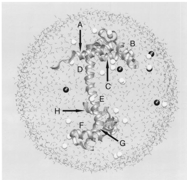
FIGURE 1 Orthographic projection of calmodulin (ribbon) from the crystal structure (Babu et al., 1988), with bound \text{Ca}^{2+} (grey) embedded in a 44-Å radius sphere of 10,474 water molecules (outer 4-Å shell shown). Twenty-two \text{Na}^+ (white) and 6 \text{Cl}^- ions (black) were placed to neutralize the system at physiological ionic strength. The eight \alpha -helices, comprising residues 5–19 (helix A), 29–38 (helix B), 45–55 (helix C), 65–78 (helix D), 82–92 (helix E), 102–111 (helix F), 118–128 (helix G), and 138–147 (helix H), are indicated. The structure is visualized with the molecular graphics program VMD (Humphrey et al., 1996).
