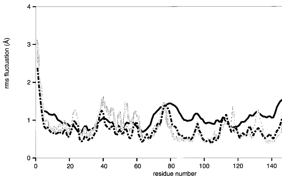
FIGURE 5 Comparison of rms fluctuations from simulation and from crystallographic B -factors (Babu et al., 1988; solid, black). Fluctuations computed individually for the N-terminal domain (res. 1–77) and C-terminal domain (res. 78–148) sampled from 0–1 ns (dashed, grey), 1–2 ns (solid, grey), and 2–3 ns (dashed, black) are shown.
